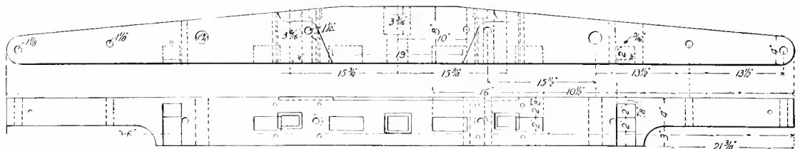
Figs. 1221-1222. Platform End-timbers (2).
